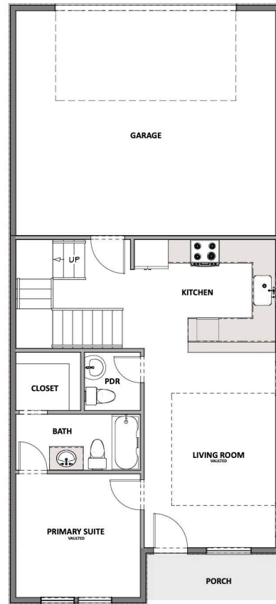
MAN FLOOR Approx 729 Sq. Ft
